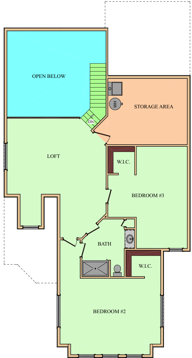
Second Floor
